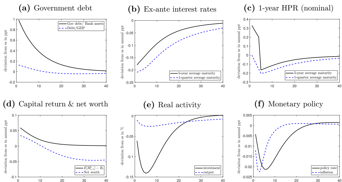
Figure C.4: Impulse responses to recession shock under Regime M
