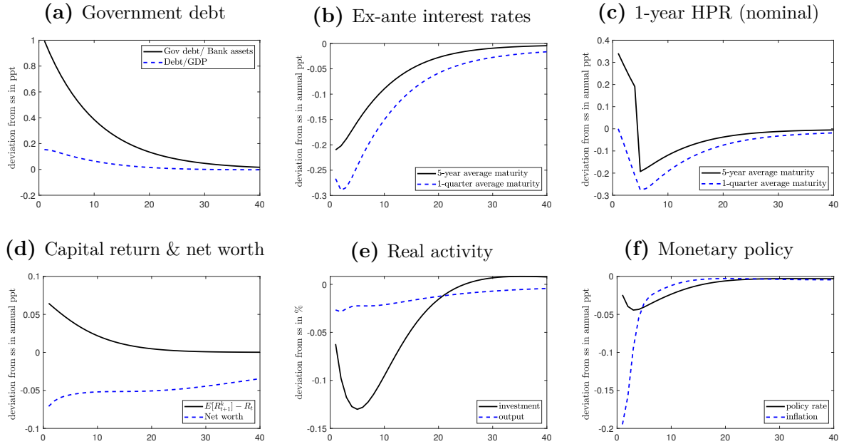
Figure 5: Impulse responses to recession shock
