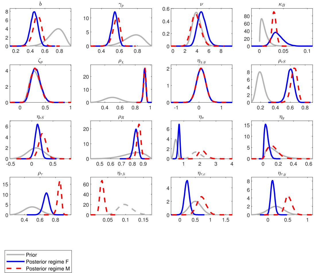
Figure C.2: Prior and posterior plots
