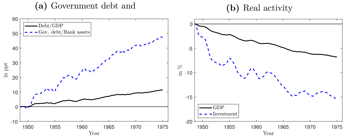
Figure D.2: Quantifying the difference under regime M due to repression for ...
